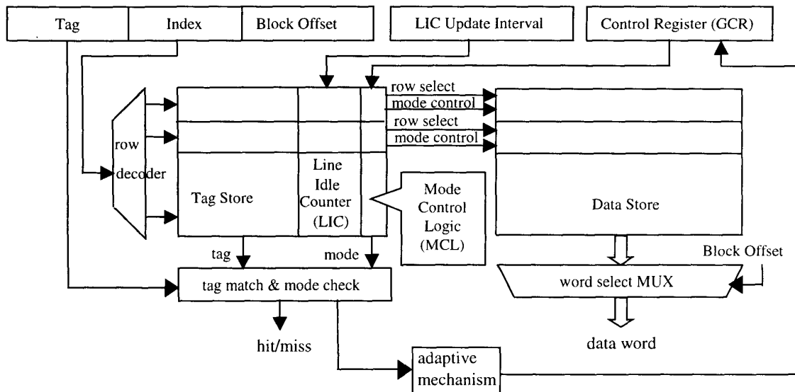
Figure 2. AMC cache architecture (direct mapped cache shown).
