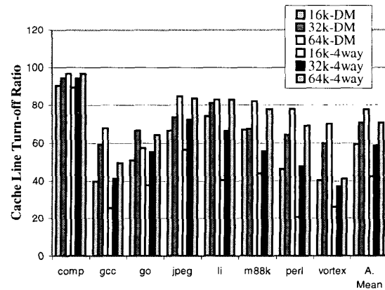
Figure 8. AMC I-Cache: Turn-off Ratio.
