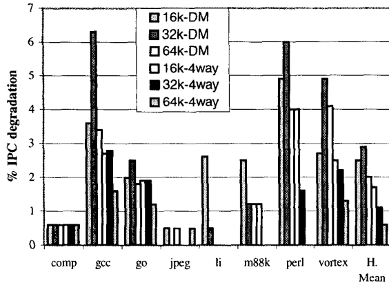
Figure 7. AMC I-cache: performance degradation.
