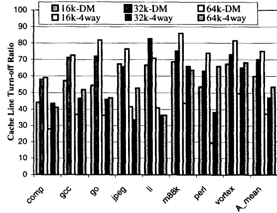
Figure 10. AMC D-cache: Turn-off Ratio.
