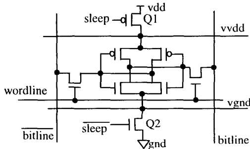
Figure 6. SRAM cell with sleep mode support.
